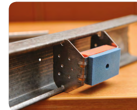
Trillingswerende beugel
